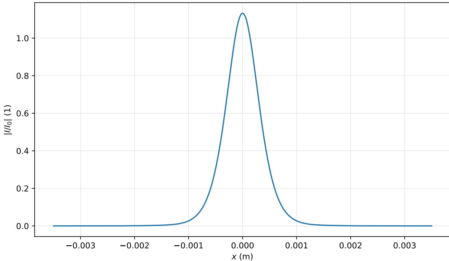
Intensity profile I(x, y = 0, z = 2.866m)/I_0 , P_{in}=0.8P_{cr} , artificial time
